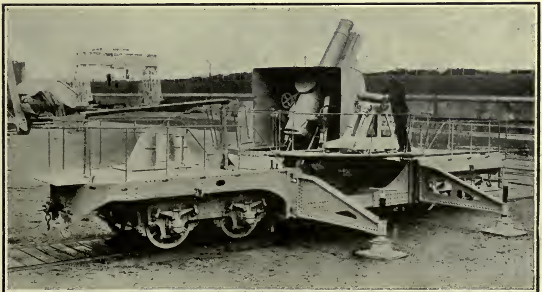
FRENCH MOVABLE HOWITZER FORTRESS.
